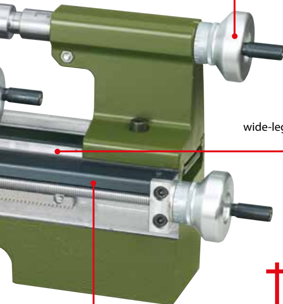
Protected lead screw with 12 x 1.5 Acme thread.
