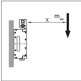
▲ Wandmontage
