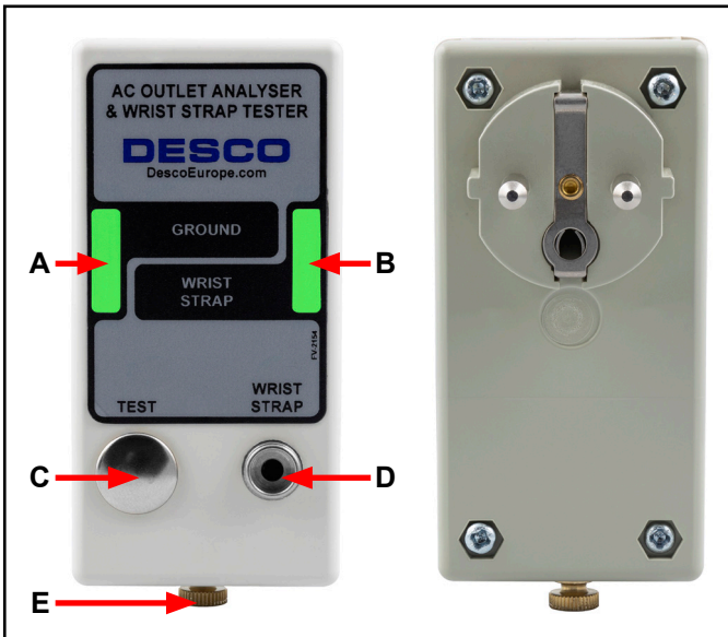
Figure 4. 98135 AC Outlet Analyser and Wrist Strap Tester features and components
