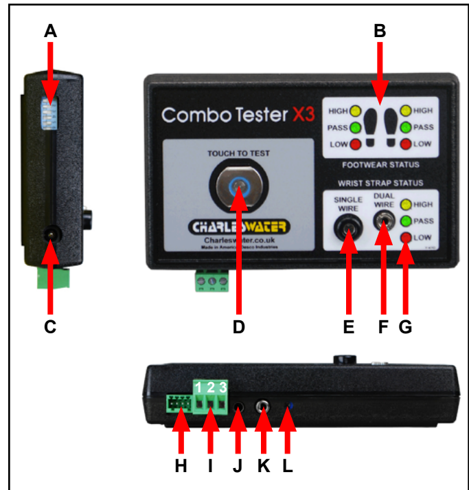
Figure 2. Charleswater Combo Tester X3 features and components
