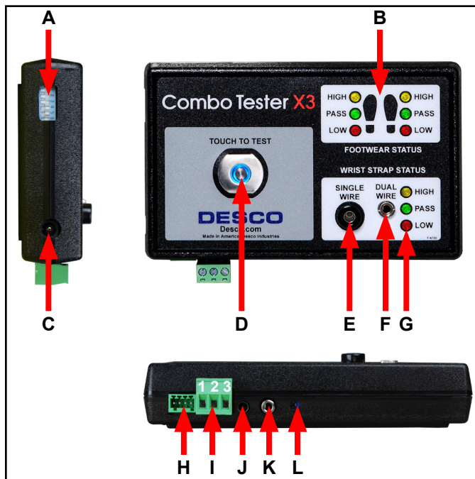
Figure 2. Combo Tester X3 features and components
