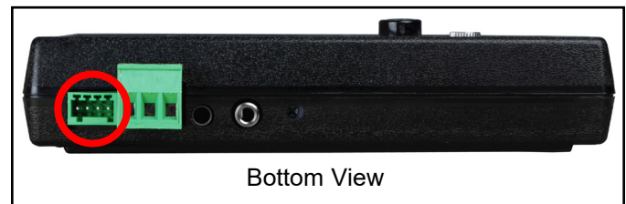
Figure 2. Locating the external test switch port on the Combo Tester X3
