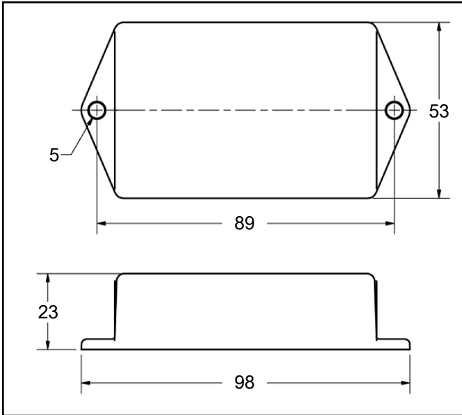
Figure 11. Mounting hole locations on the Multi-Mount Continuous Monitor (all dimensions are in mm)
