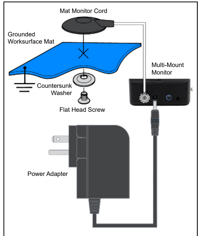
Figure 5. Installing the Multi-Mount Continuous Monitor
