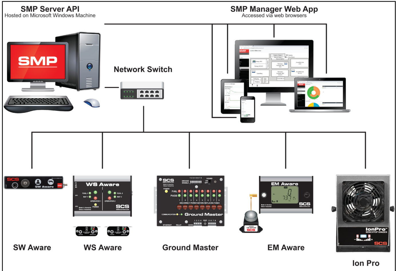
Figure 12. SMP system setup
