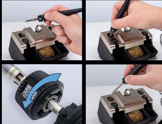
Patented tip change directly in the holder
