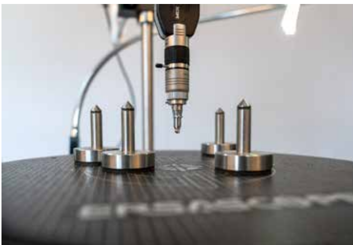
BGA inspection head with four PCB supports to handle double-sided assemblies
