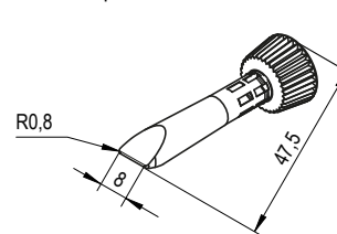
0102CDLF080C/SB chisel-shaped, conical, 8.0 mm
