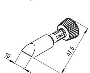
0102CDLF100/SB chisel-shaped, 10.0 mm
