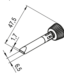
0102CDLF65/SB chisel-shaped, 6.5 mm
