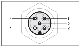
Schematic drawing of M12 plug
