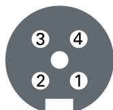
PIN 3 GND PIN 4 V DC
