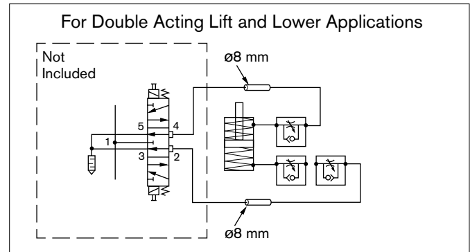
Pneumatic diagram for HQ2/E, HQ2/U, EQ2/T*, EQ2/TE*
