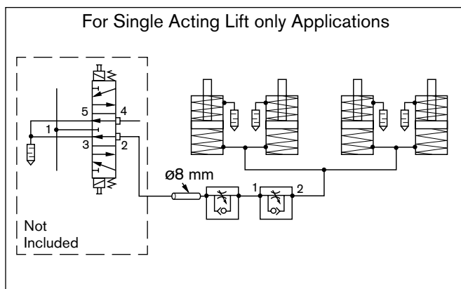
Pneumatic diagram for HQ2/U3
