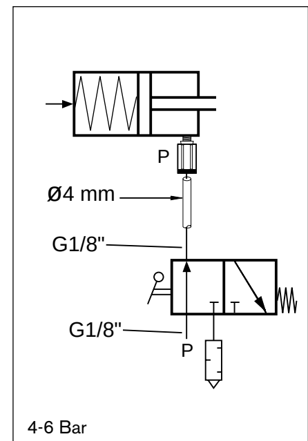
Pneumatic diagram, VE2/WI
