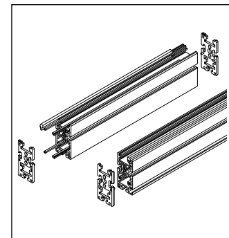
ST2/R-H Vplus Conveyor Section Profiles 6-6 to 6-7
