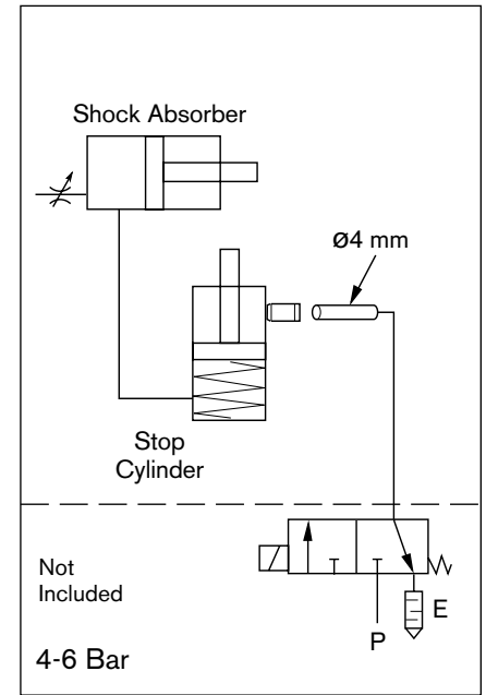
Pneumatic diagram, VE2/D20, VE2/D60
