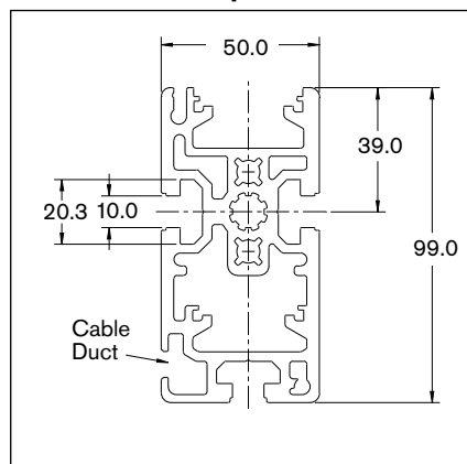
H.D. Flat-Top Chain Profile
