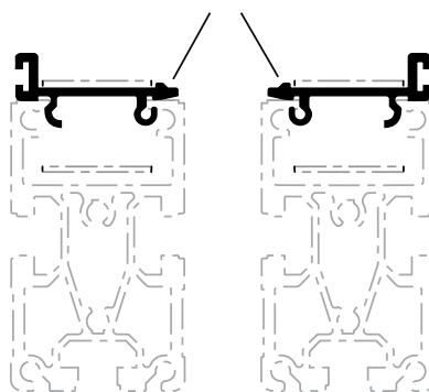
FP2/B Belt Guide Profile (shown with SP2/B conveyor profile)
