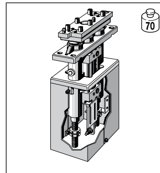
HP2 Lift-position Unit 13-4 to 13-5
