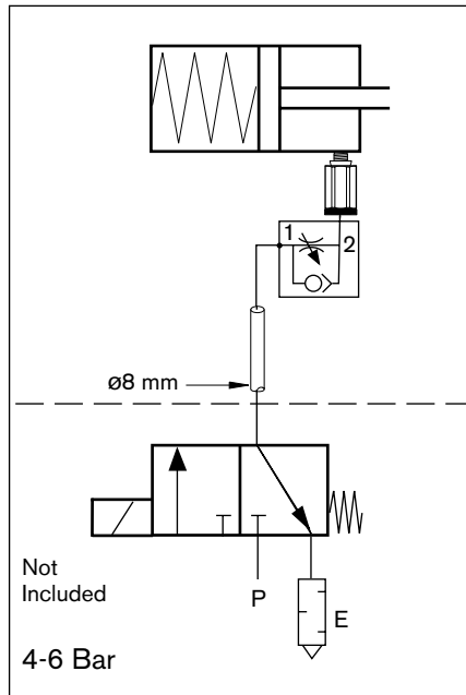
Pneumatic diagram, VE2/H
