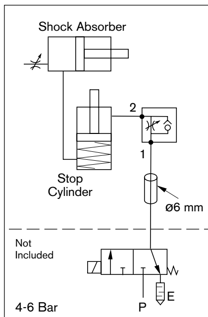
Pneumatic diagram, VE2/D200
