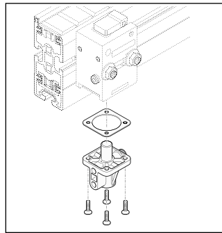
VE2 Positioning Sensor Kit 15-2
