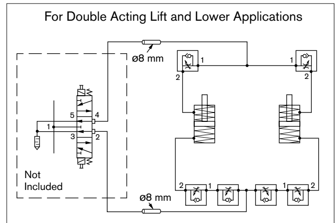
Pneumatic diagram for EQ2/TR*, EQ2/T*, EQ2/TE*
