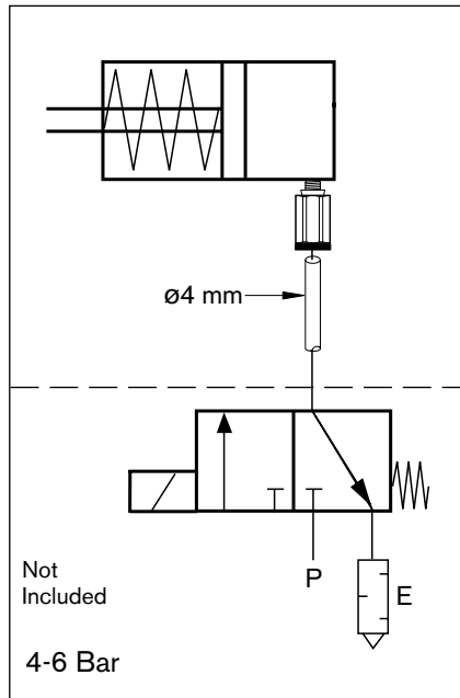
Pneumatic diagram, VE2/VA
