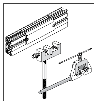
ST2/C-W Maintenance, Module and Flat-top Chain Tools 4-16
