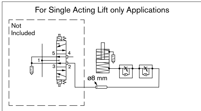
Pneumatic diagram for HQ2/E, HQ2/U, EQ2/T*, EQ2/TE*
