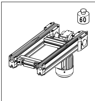
BS2 Transverse Conveyors 9-2 to 9-3
