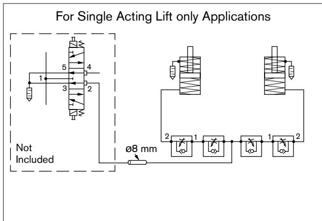
Pneumatic diagram for EQ2/TR*, EQ2/T*, EQ2/TE*
