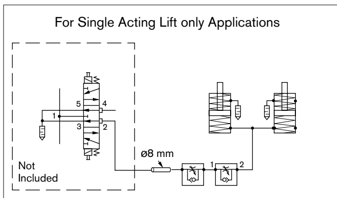
Pneumatic diagram for HQ2/U2
