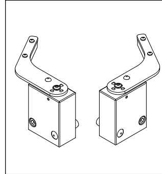
CW2 Conveyor Wiper Kit 7-2
