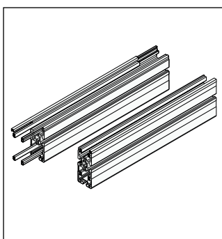
ST2/C, CRV2/1, CRV2/2 Straight and Curved Conveyor Sections 4-9 to 4-13
