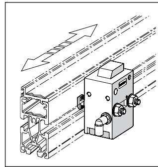
VE2/S Bi-Directional Stops 15-3
