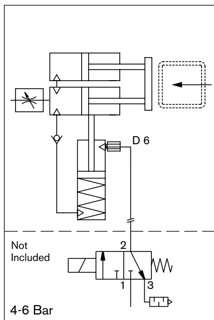
Pneumatic diagram, VE2/D150
