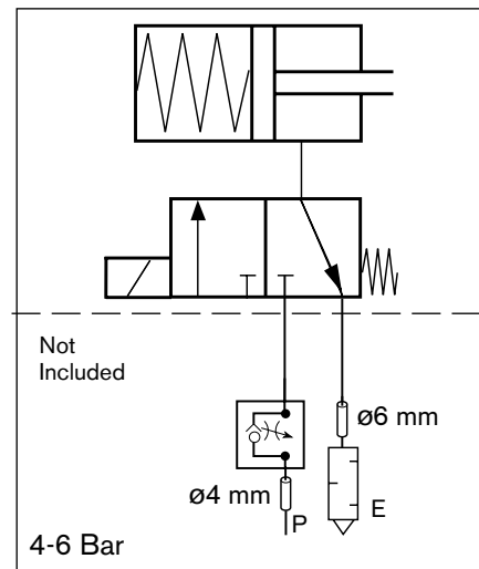
Pneumatic diagram, VE2/MP
