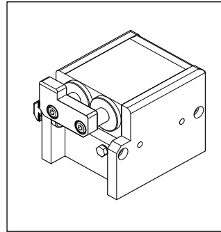
VE2/D-150 Cushioned Stop 15-8 to 15-9
