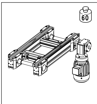
BS2/K Transverse Conveyors 9-10 to 9-11
