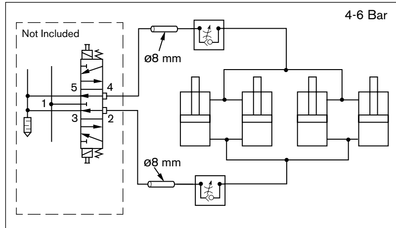
Pneumatic diagram for PE2/X
