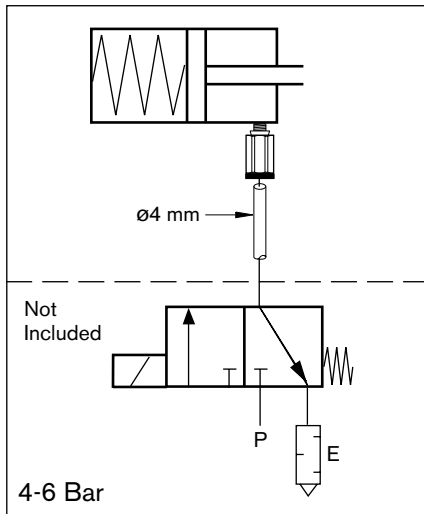
Pneumatic diagram, VE2, VE2/L, VE2/M, VE2/S
