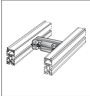
QV2 Cross Connectors 7-1
