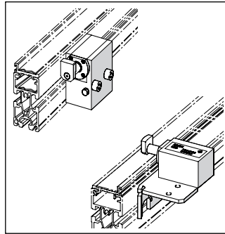
VE2/... Cushioned Stops 15-6 to 15-7
