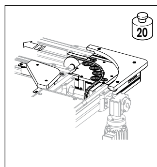
KE2/90-0 Slave Driven 10-1
