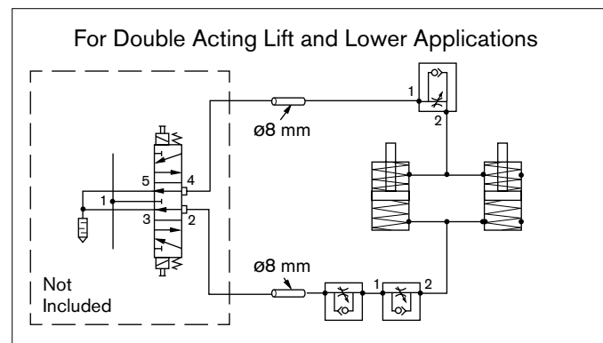
Pneumatic diagram for HQ2/U2
