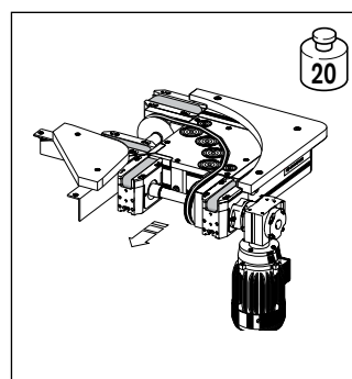
KE2/90 90° Powered Curve 10-4 to 10-5
