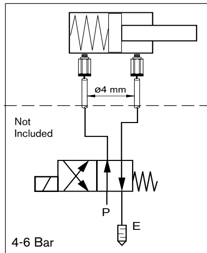
Pneumatic diagram, VE2/D
