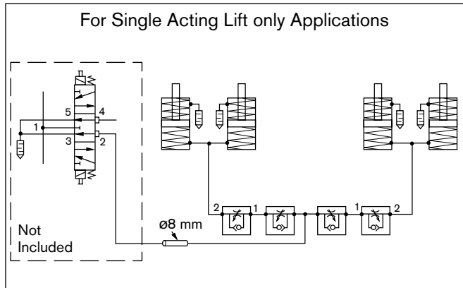
Pneumatic diagram for EQ2/TR*, EQ2/T*, EQ2/TE*
