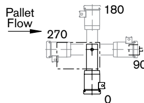
Outboard Mounted Motor Orientation
