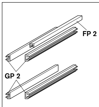
FP2/R, FP2/C Roller & Flat-Top Chain Guide Profile 7-7
