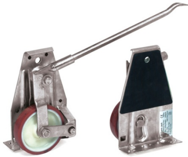
Lifting rolls
